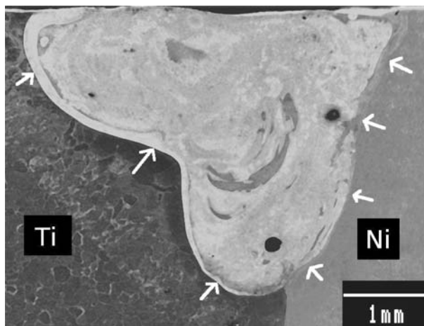
Figure 2 Low magnification image showing the asymmetric weld pool. Fusion interfaces are shown by arrows.
