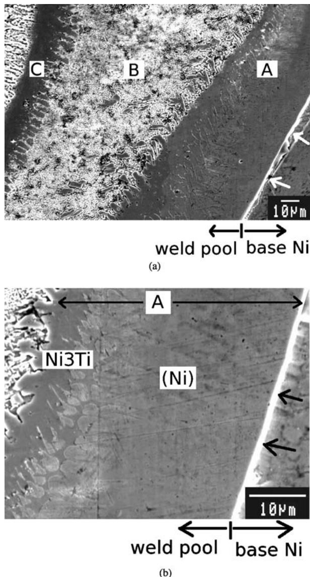
Figure 4 (a) The figure reveals the formation of bands at the Ni fusion interface. (b) Band 'A' is made up of (Ni) and Ni 3 Ti layers. Arrows show the fusion interface in both (a) and (b). (c) Bands 'B' and 'C'. Ni 3 Ti+NiTi eutectic and some primary Ni 3 Ti faceted dendrites appear in 'B' (magnified views of these are shown in the top of the figure). 'C' is a layer of NiTi from which cellular growth is observed both in the direction of 'B' as well as toward the weld pool.
