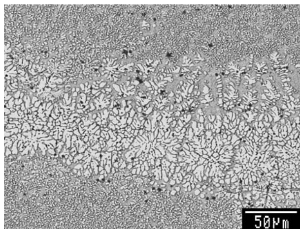
Figure 6 BSE image showing alternate layers of coarse and fine NiTi structures which appear throughout the central region of the weld. Ti_2Ni phase is spread across these layers.
