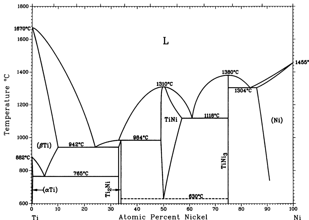
Figure 1 The Ti-Ni phase diagram.
