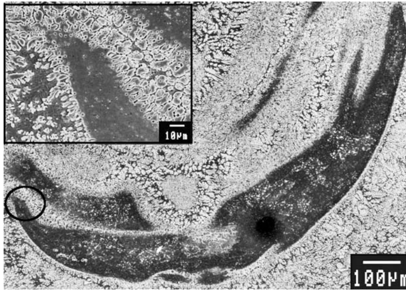
Figure 7 Large NiTi blocks appear mostly near the bottom of the weld pool. Cellular growth from the periphery of the blocky NiTi is shown in the inset.
