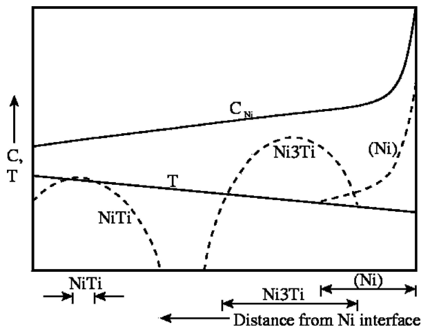
Figure 10 Schematic illustration of the variation of temperature, composition and liquidus temperature near Ni fusion interface.
