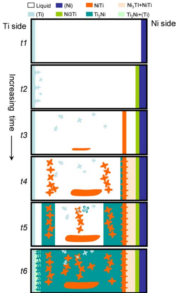
Figure 11 A schematic diagram depicting the evolution of different phases during the solidification of molten weld pool obtained during the laser welding of Ti and Ni. The snapshots at increasing times are presented from top toward bottom. Colormaps indicate the phases. See text for details.
