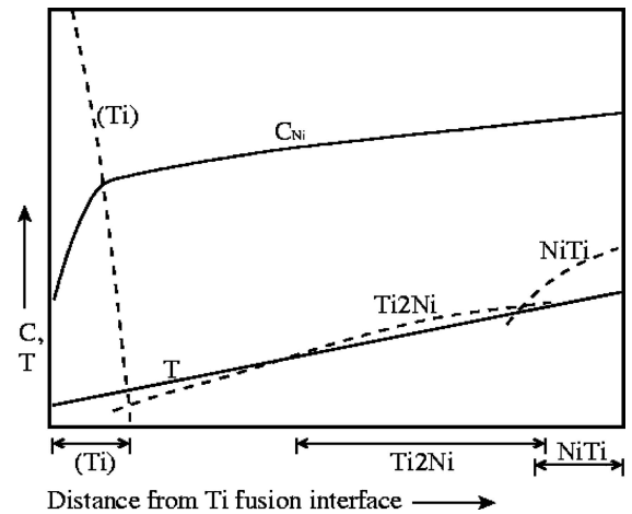
Figure 9 Schematic illustration of the variation of temperature, composition and liquidus temperature near Ti fusion interface. Firm lines represent the temperature and composition in the melt and the dashed lines are for the liquidus temperatures of the respective phases (indicated in the figure).
